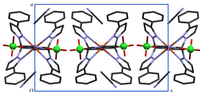
Figure 2 The packing of [\text{CuL}_2](\text{ClO}_4)_2 \cdot 2\text{C}_2\text{H}_3\text{N} , viewed along the c axis.
